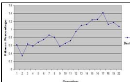
Fig.7 showing fitness of the population graph for bufferoverflow attack
