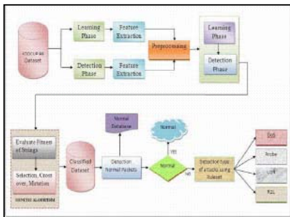
Fig. 2: The simple Architecture of the proposed model
