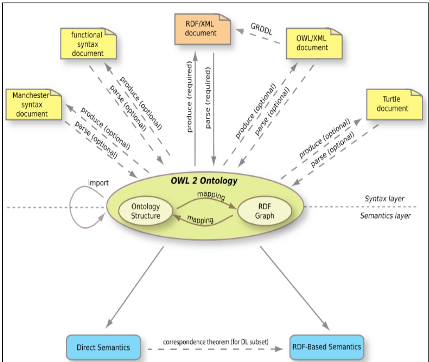
Fig. 2: Structure of OWL 2
