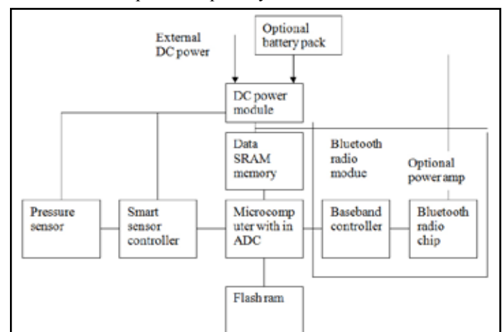
Fig. 4: Bluetooth Wireless Smart Pressure Sensor Node
