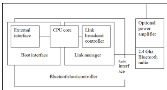
Fig. 5: Bluetooth Module Hardware Architecture
