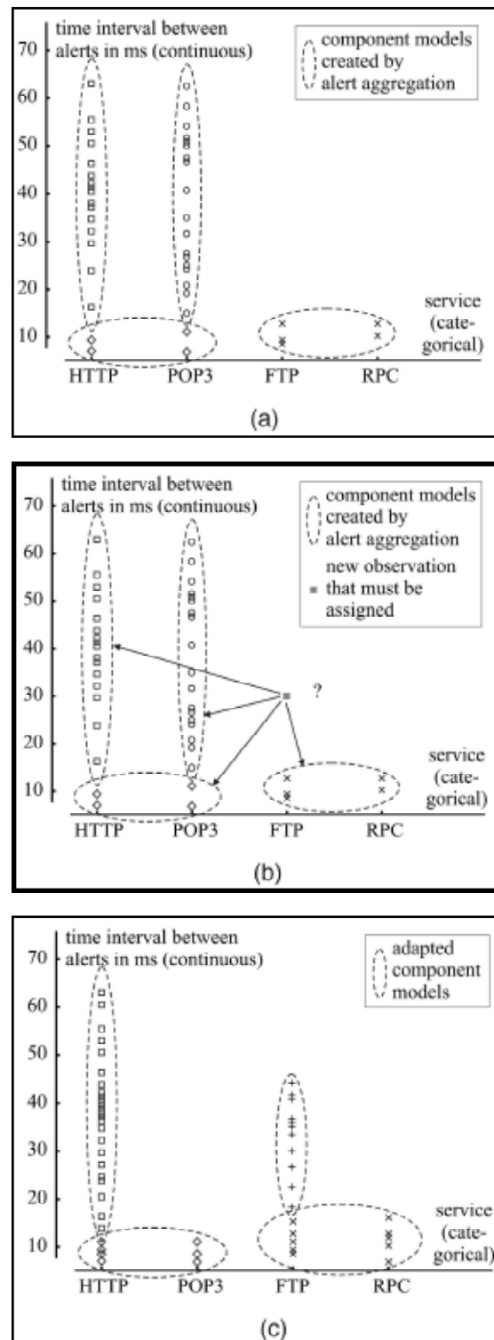
Fig. 2: Example Illustrating the Principle of online alert aggregation
