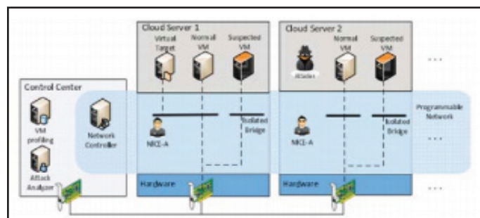
Fig. 1: Nice Architecture with One Cloud Server
