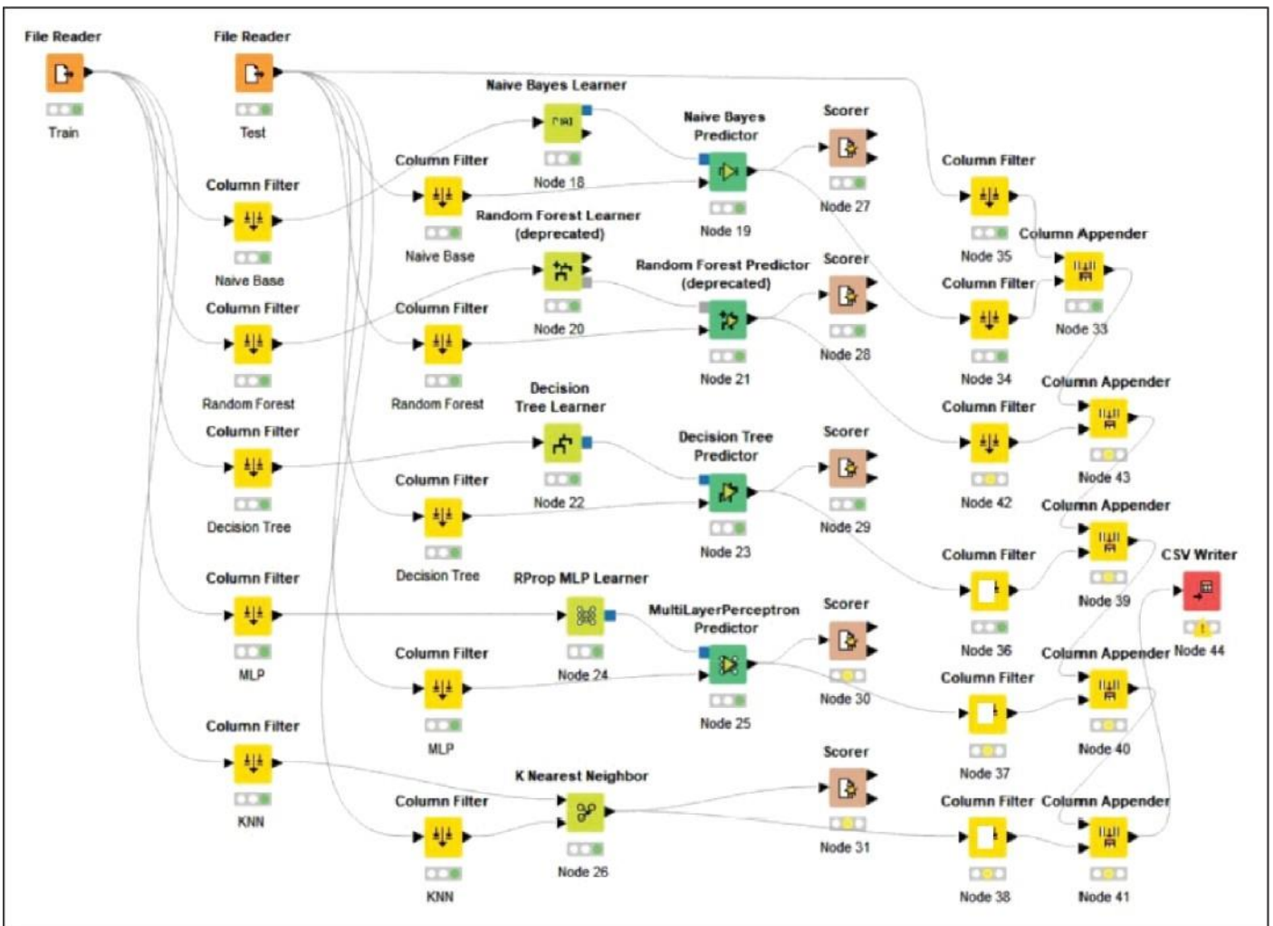
Fig. 3: KNIME Workflow Diagram
