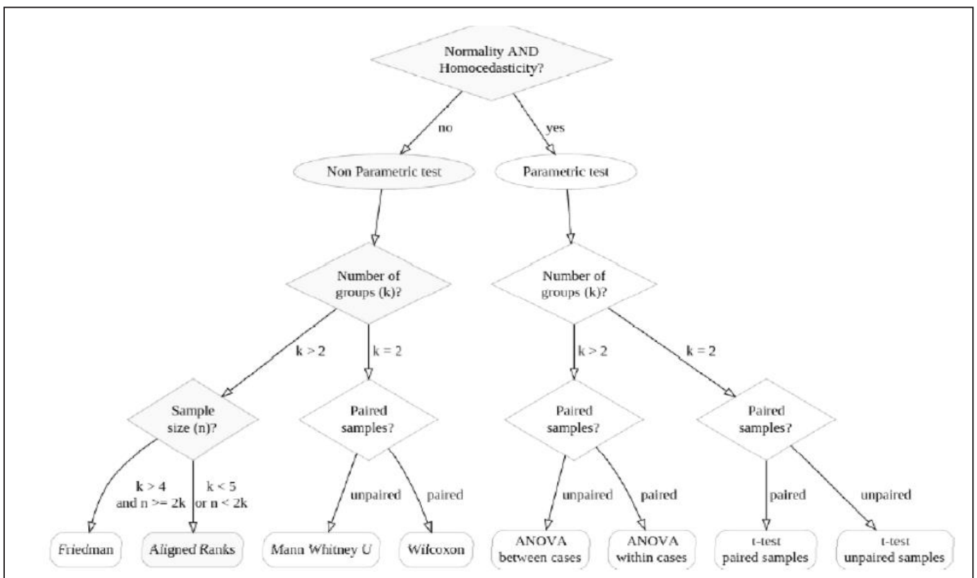
Fig. 6: STAC Assistant Decision Tree [35].
