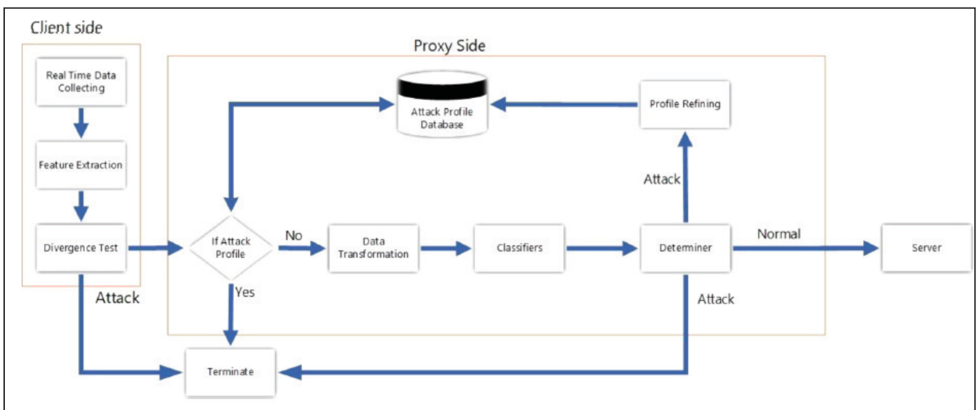
Fig. 1: The proposed framework.
