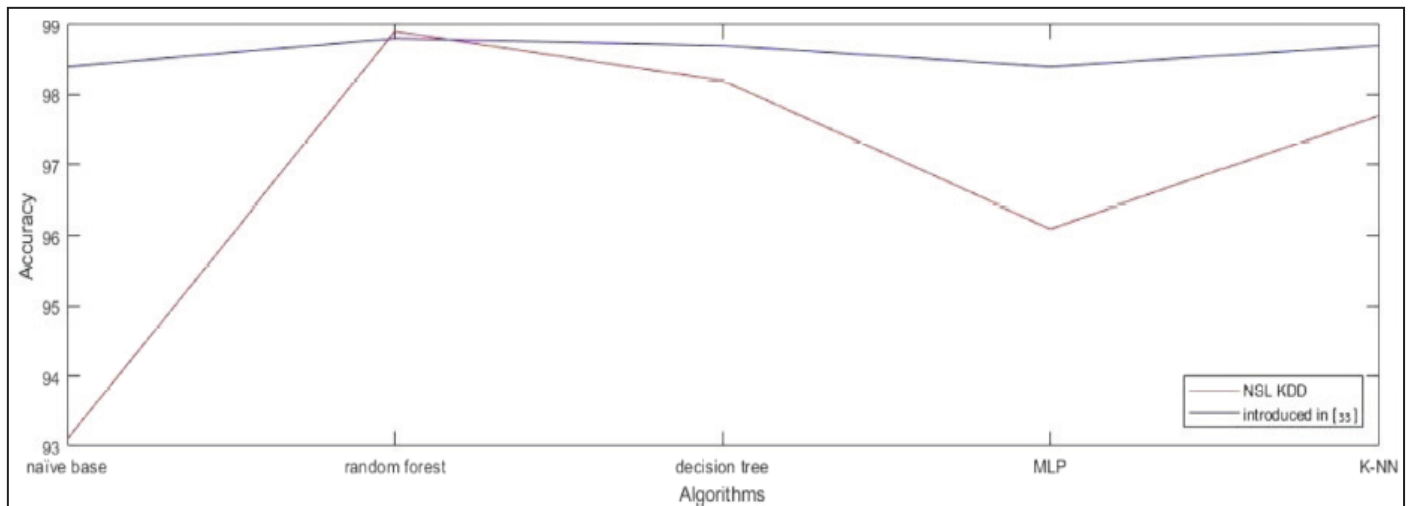
Fig. 5: Accuracy Compare Between Algorithms for two datasets.
