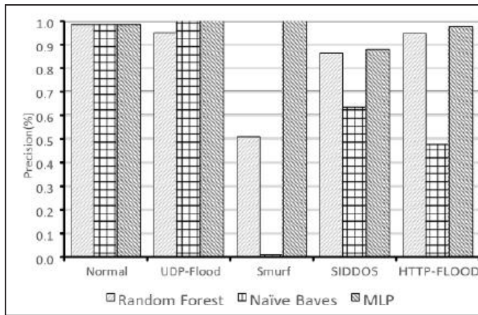
Fig. 10: Precision Results
