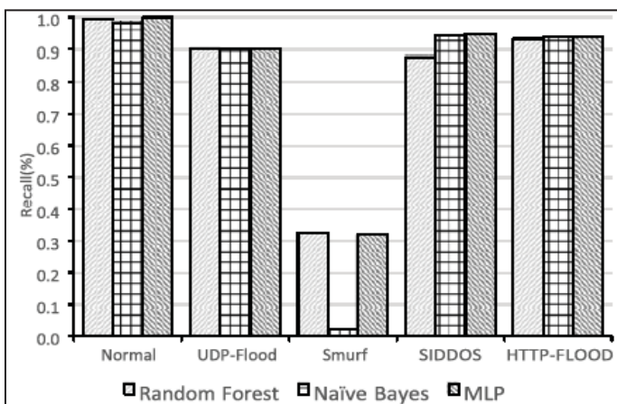
Fig. 11: Recall Results
