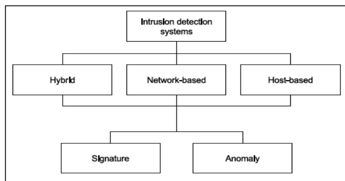
Fig. 2: IDS Classification
