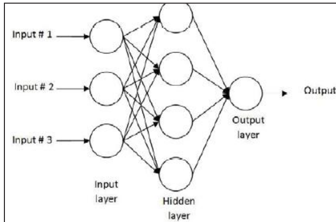
Fig. 8: MLP Structure
