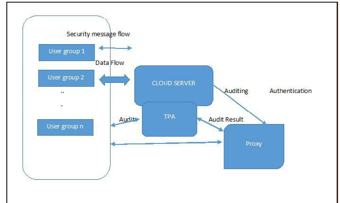
Fig. 2 Cloud Regeneration Architecture
