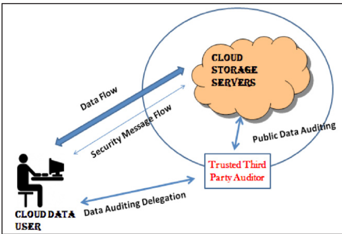
Fig. 1: The Architecture of Cloud Data Storage Services
