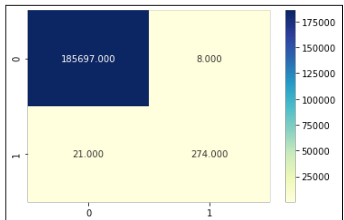
Fig. 9: Confusion matrix for testing dataset
