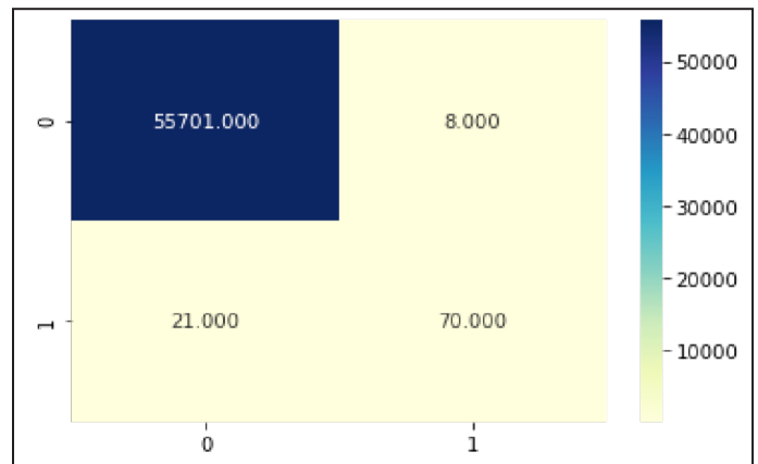
Fig. 8: Confusion matrix for testing dataset
