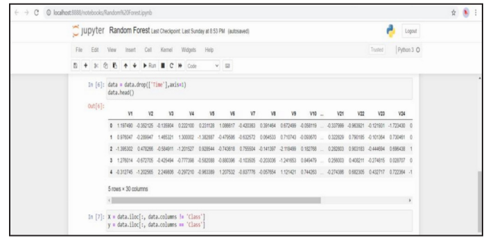
Fig. 5: Preprocessing Step 2
