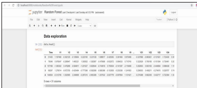
Fig. 3: Data exploration
