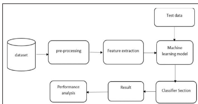
Fig. 1: System Architecture
