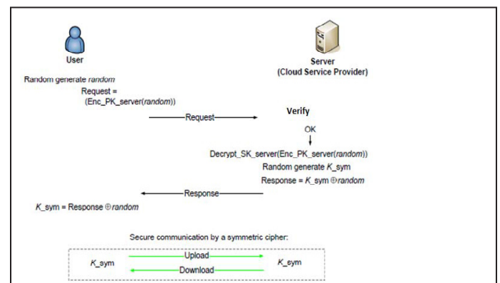
Fig. 3: Proposed Architecture diagram
